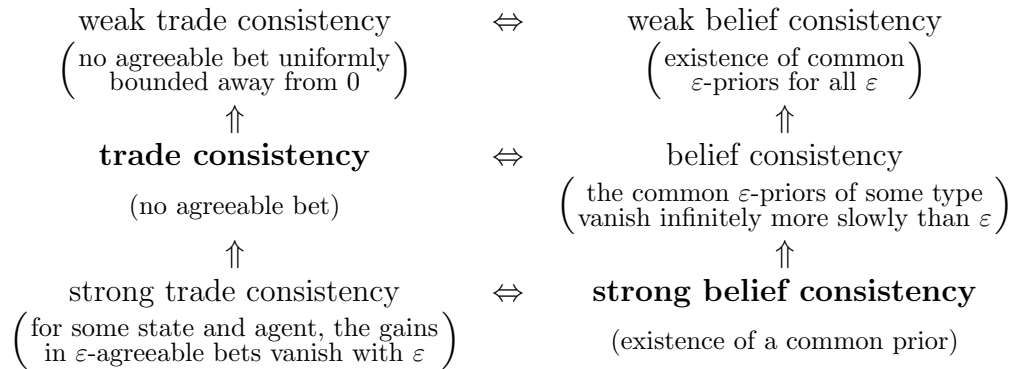
Diagram 1. Three equivalence theorems
